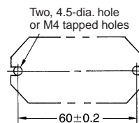
Mounting Holes
