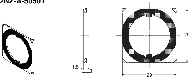
Lock Ring
