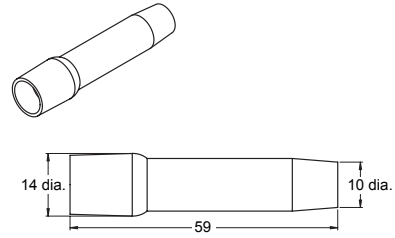
LED Extractor A22NZ-A-302
